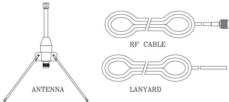
Figure 1 – Parts Diagram
