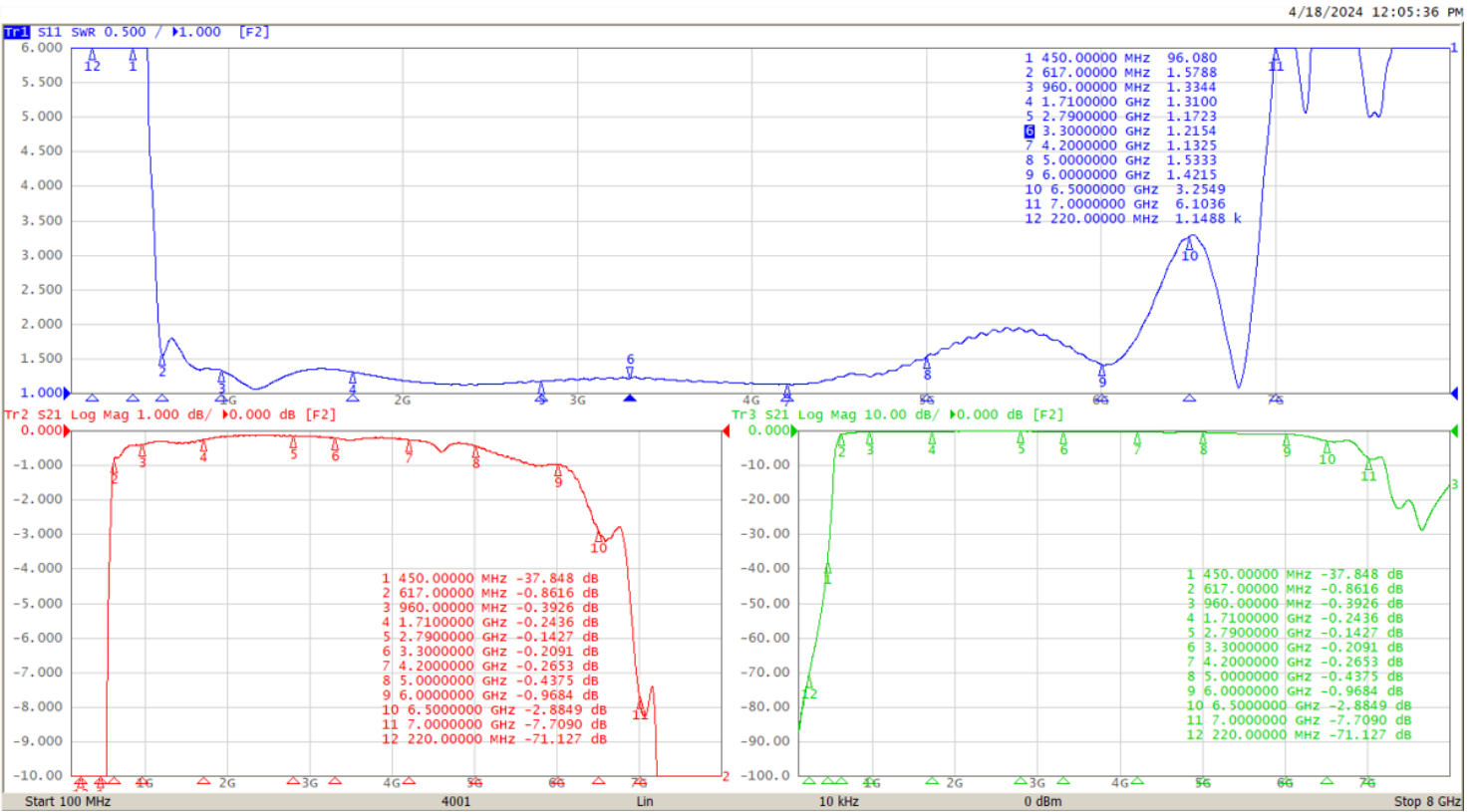
Typical Response Curve
